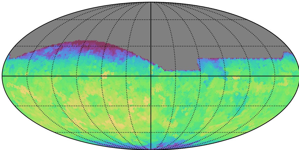
too_100_4v3.4_10yrs All sky all bands: Max fiveSigmaDepth
