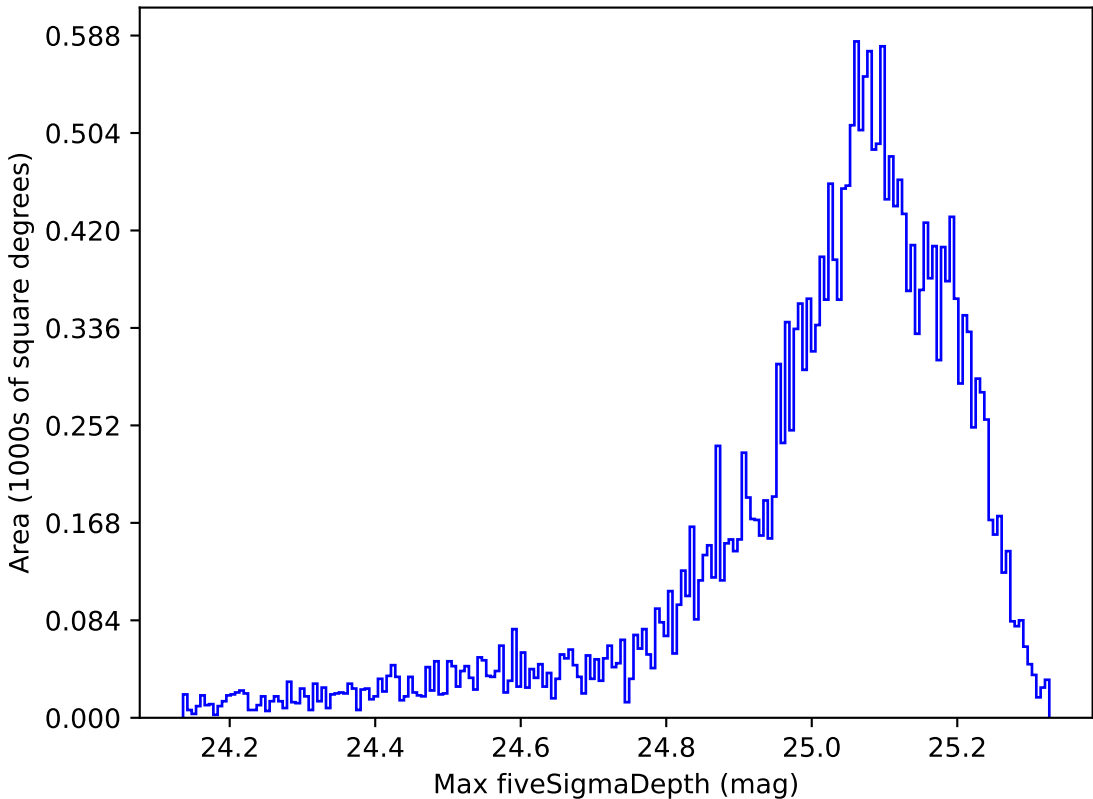
too_100_4v3.4_10yrs All sky all bands: Max fiveSigmaDepth
