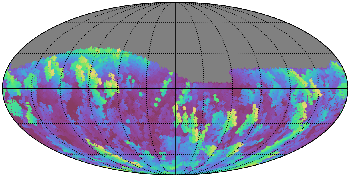
too_100_4v3.4_10yrs Yr 1 z band: Max airmass
