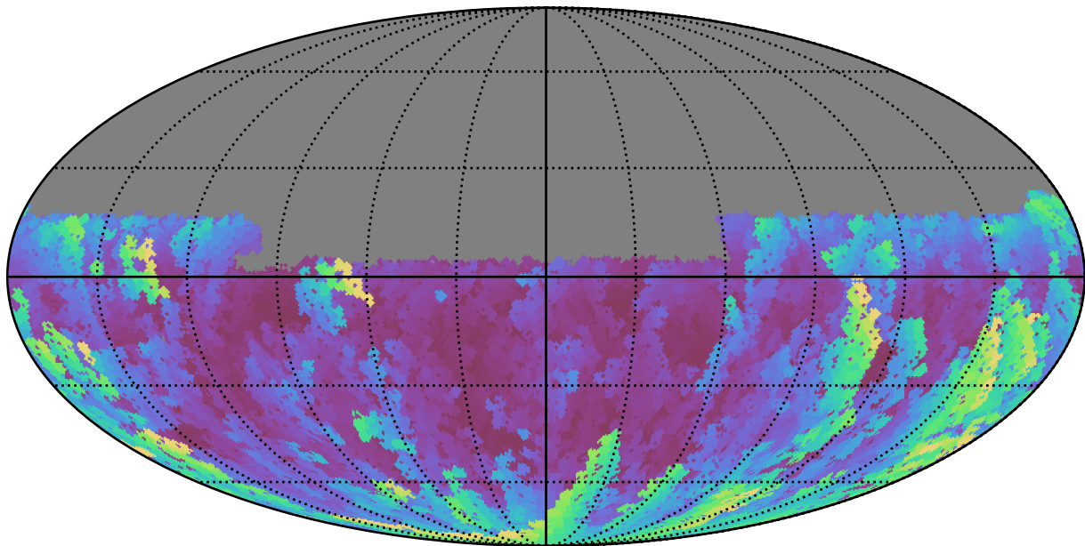
too_100_4v3.4_10yrs Yr 1 u band: Max airmass
