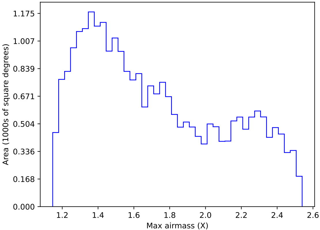
too_100_4v3.4_10yrs Yr 1 r band: Max airmass
