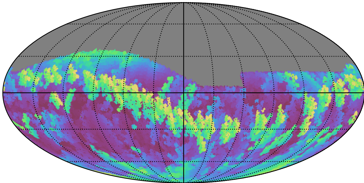
too_100_4v3.4_10yrs Yr 1 i band: Max airmass
