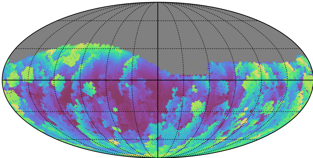
too_100_4v3.4_10yrs Yr 1 g band: Max airmass
