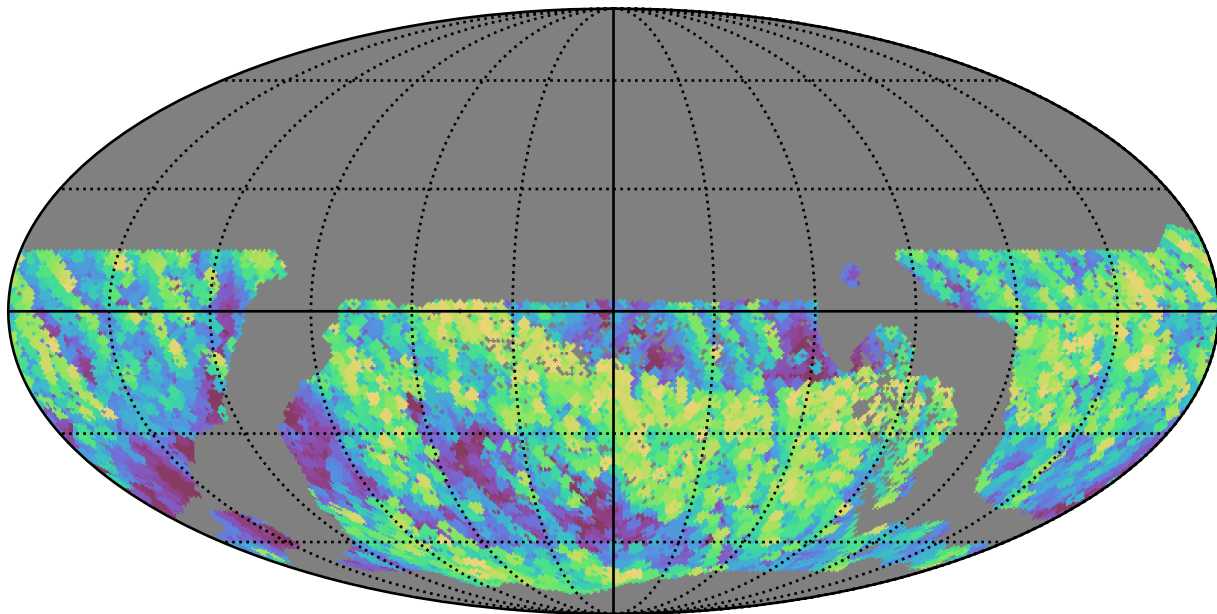
too_100_4v3.4_10yrs WFD z band: Max airmass
