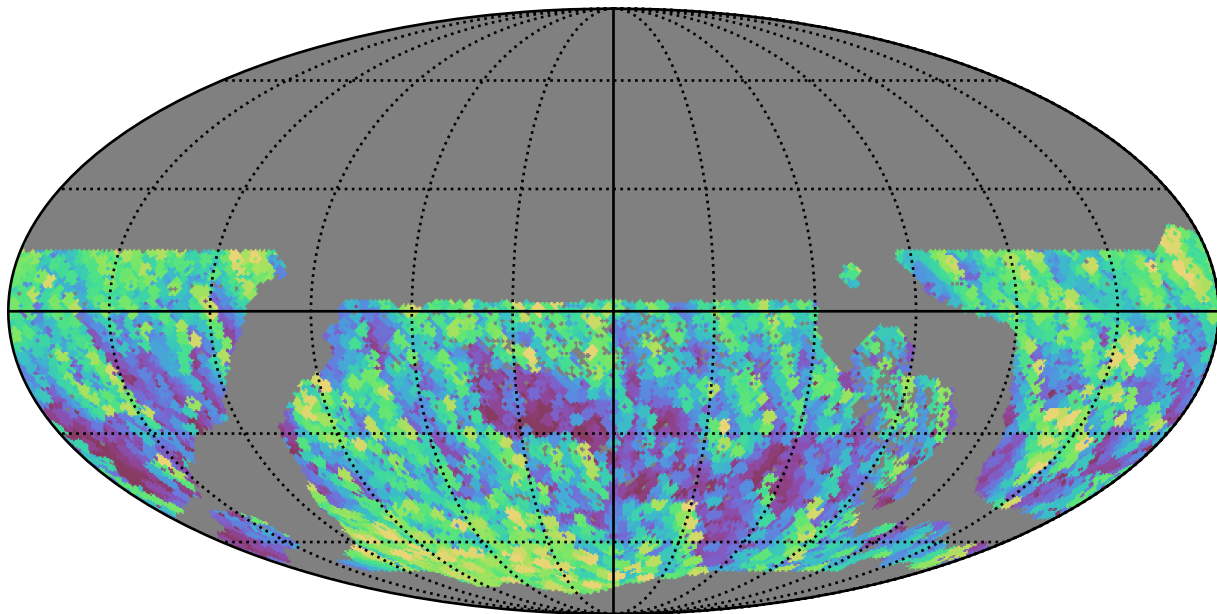
too_100_4v3.4_10yrs WFD y band: Max airmass
