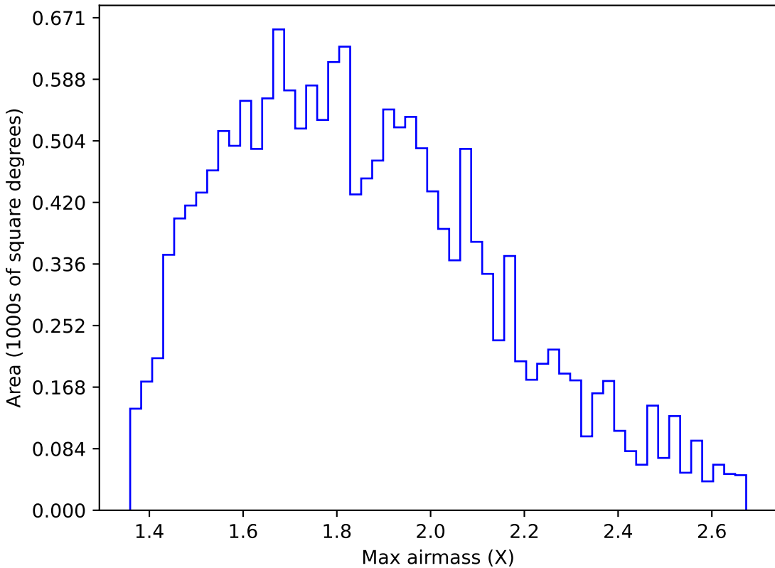
too_100_4v3.4_10yrs WFD u band: Max airmass
