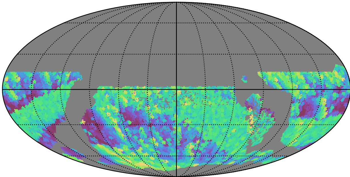
too_100_4v3.4_10yrs WFD r band: Max airmass
