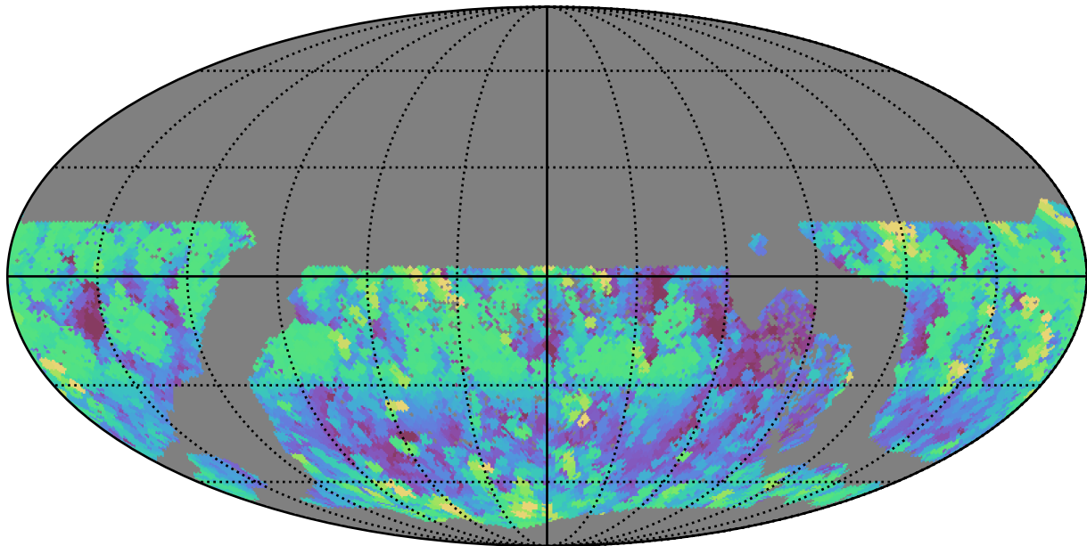
too_100_4v3.4_10yrs WFD g band: Max airmass
