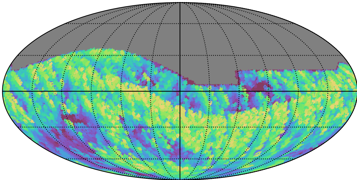
too_100_4v3.4_10yrs All sky z band: Max airmass
