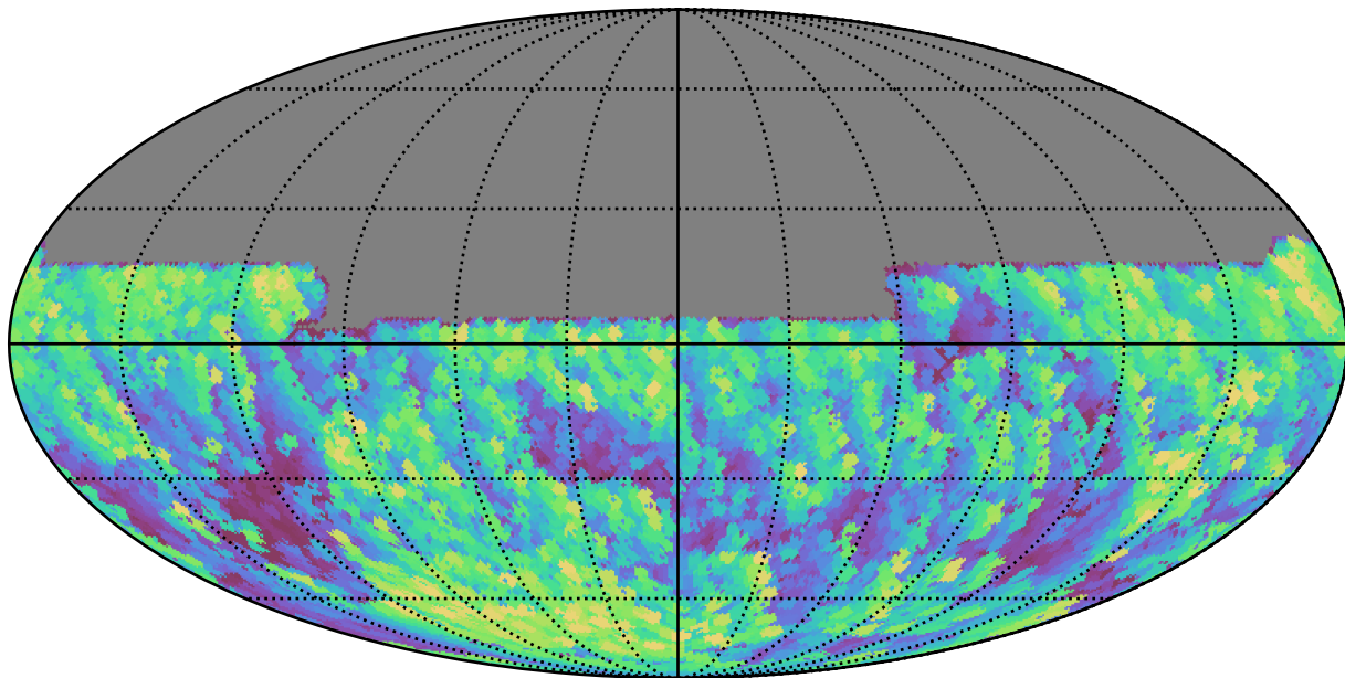
too_100_4v3.4_10yrs All sky y band: Max airmass
