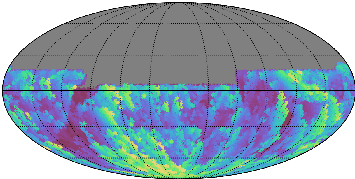
too_100_4v3.4_10yrs All sky u band: Max airmass
