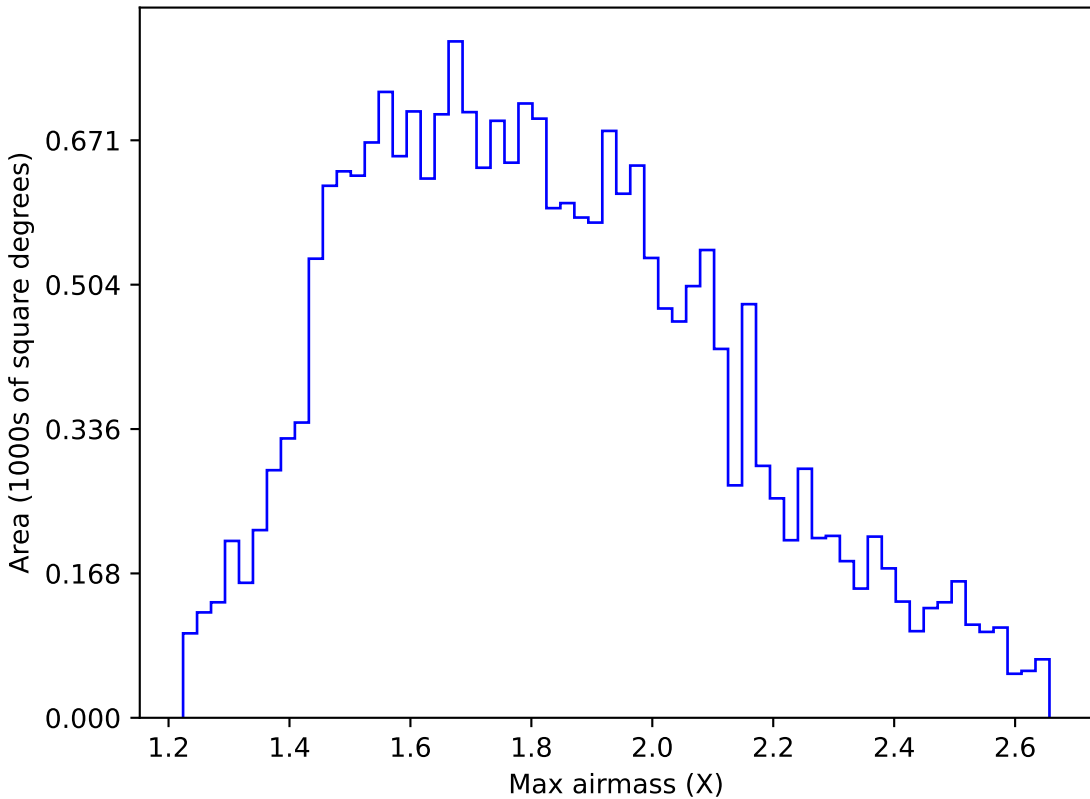
too_100_4v3.4_10yrs All sky u band: Max airmass
