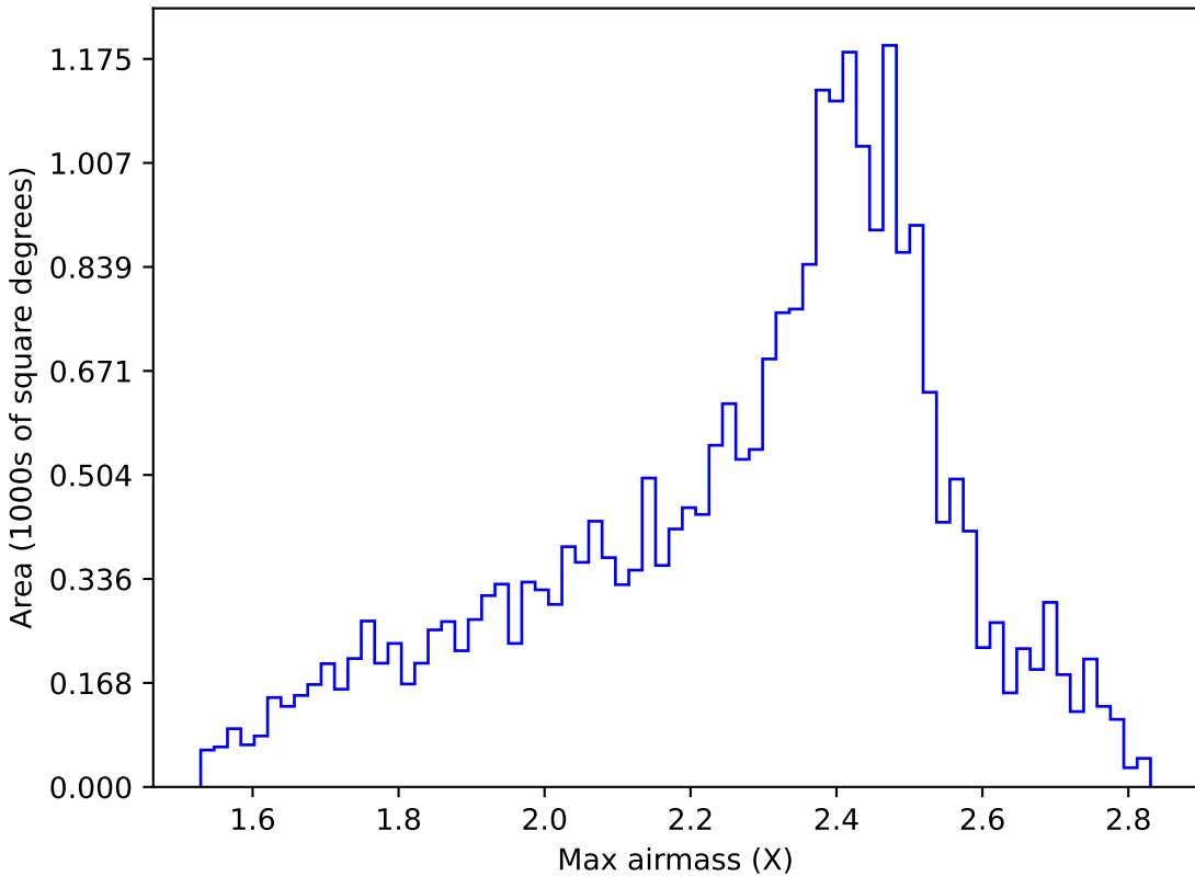
too_100_4v3.4_10yrs All sky r band: Max airmass
