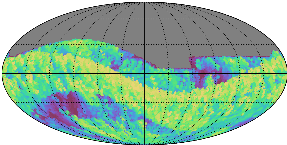
too_100_4v3.4_10yrs All sky i band: Max airmass
