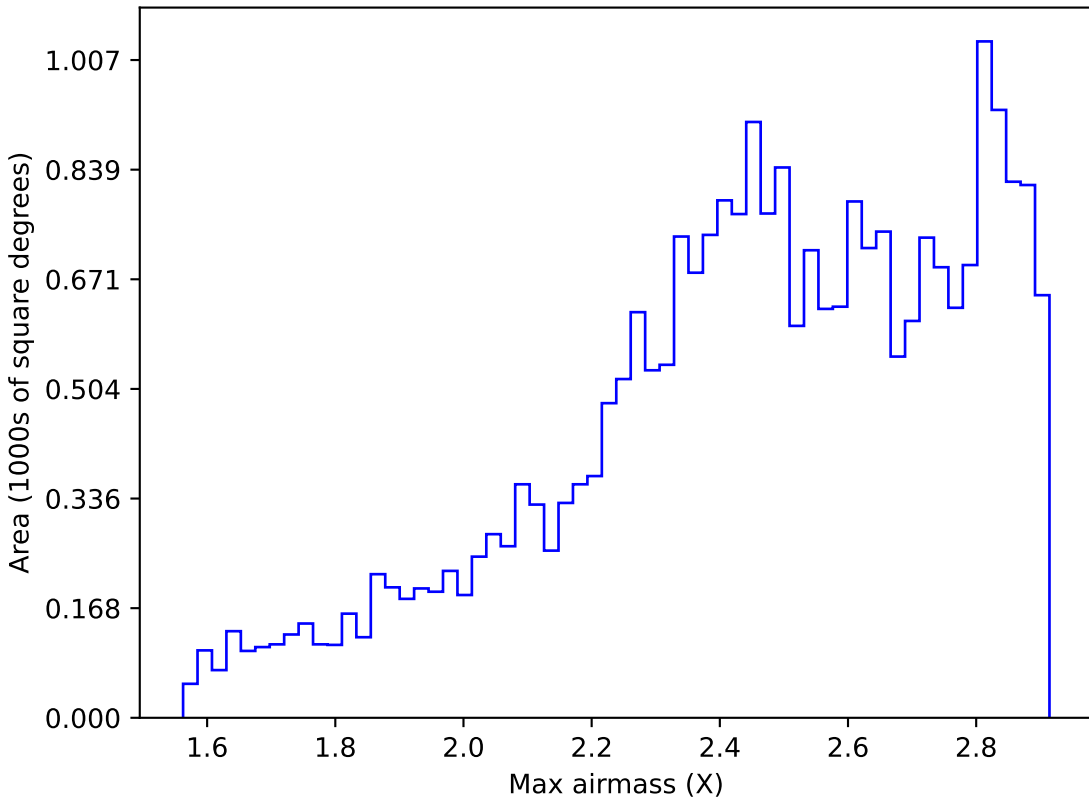
too_100_4v3.4_10yrs All sky i band: Max airmass
