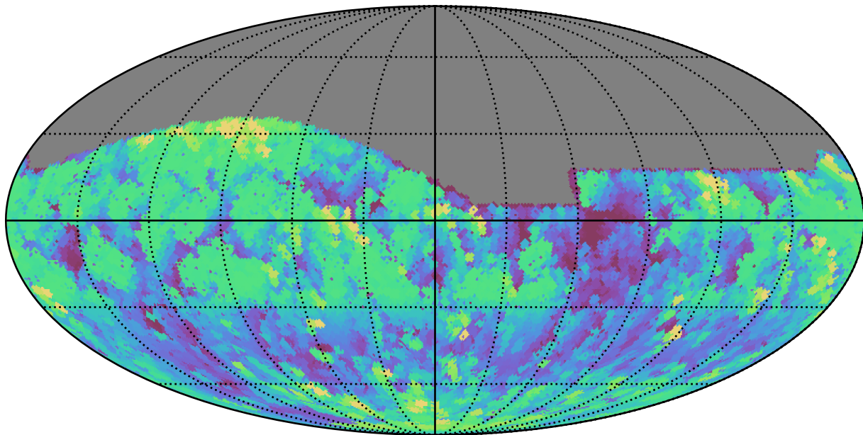
too_100_4v3.4_10yrs All sky g band: Max airmass
