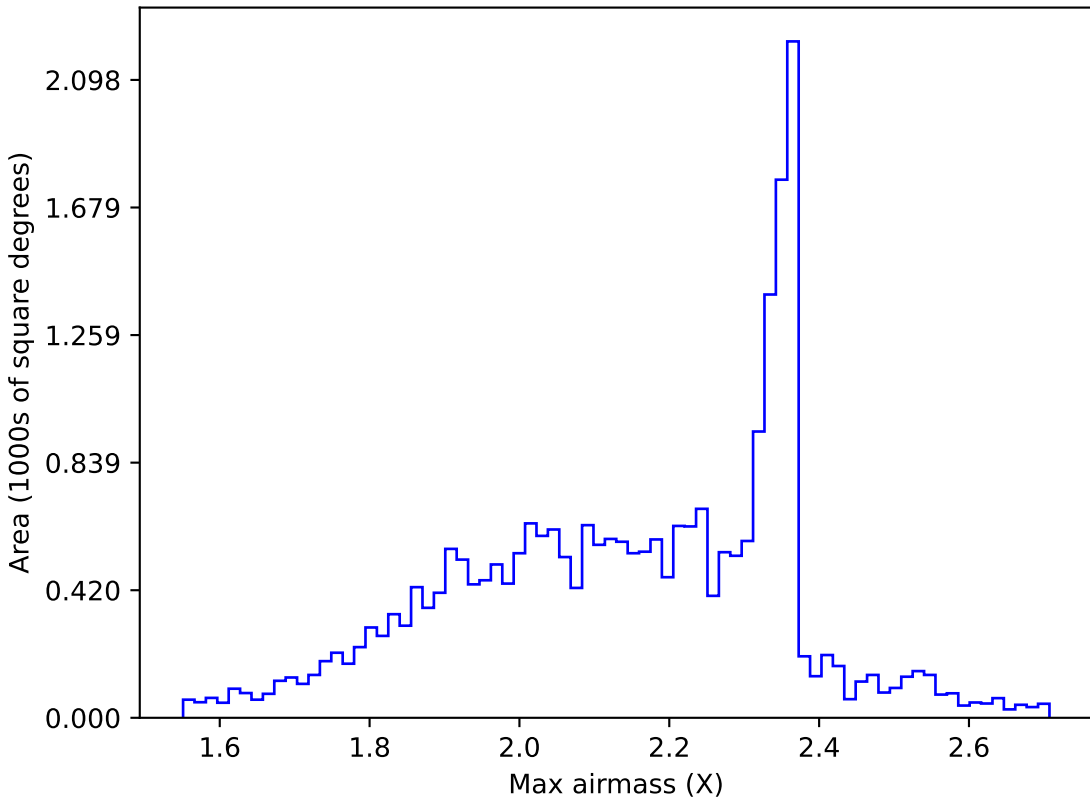
too_100_4v3.4_10yrs All sky g band: Max airmass
