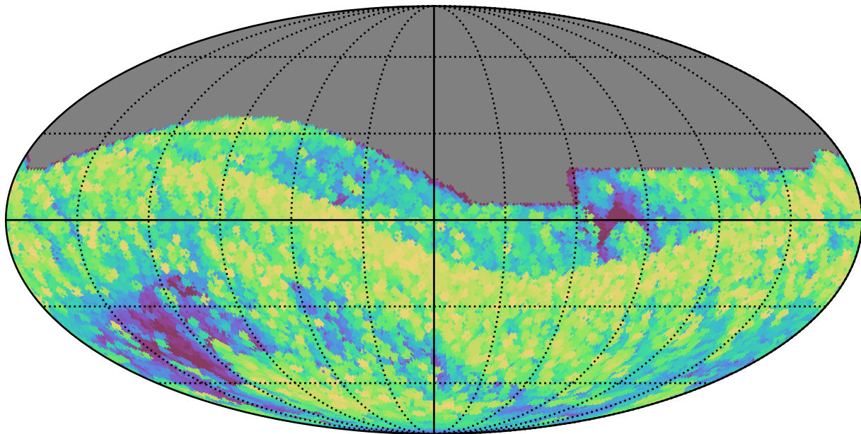
too_100_4v3.4_10yrs All sky all bands: Max airmass
