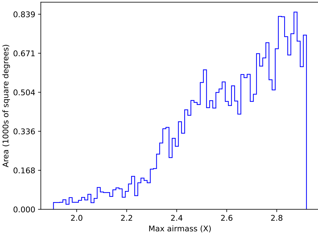
too_100_4v3.4_10yrs All sky all bands: Max airmass
