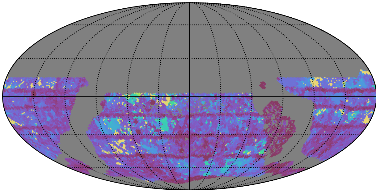
too_100_4v3.4_10yrs WFD z band: Max Inter-Night Gap
