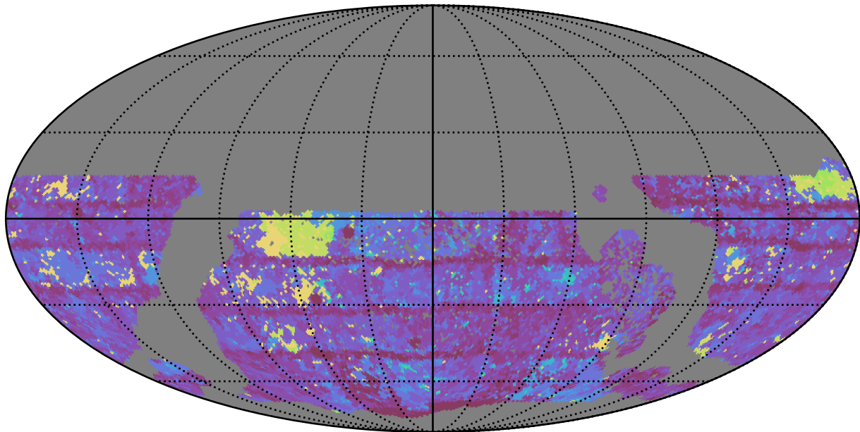
too_100_4v3.4_10yrs WFD y band: Max Inter-Night Gap
