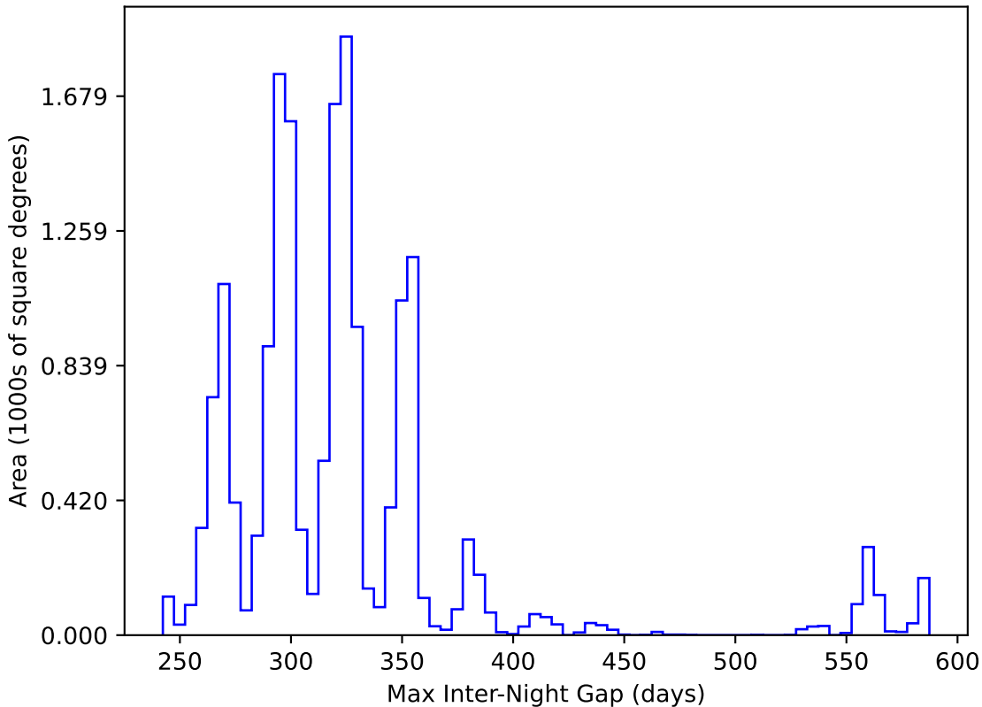
too_100_4v3.4_10yrs WFD y band: Max Inter-Night Gap
