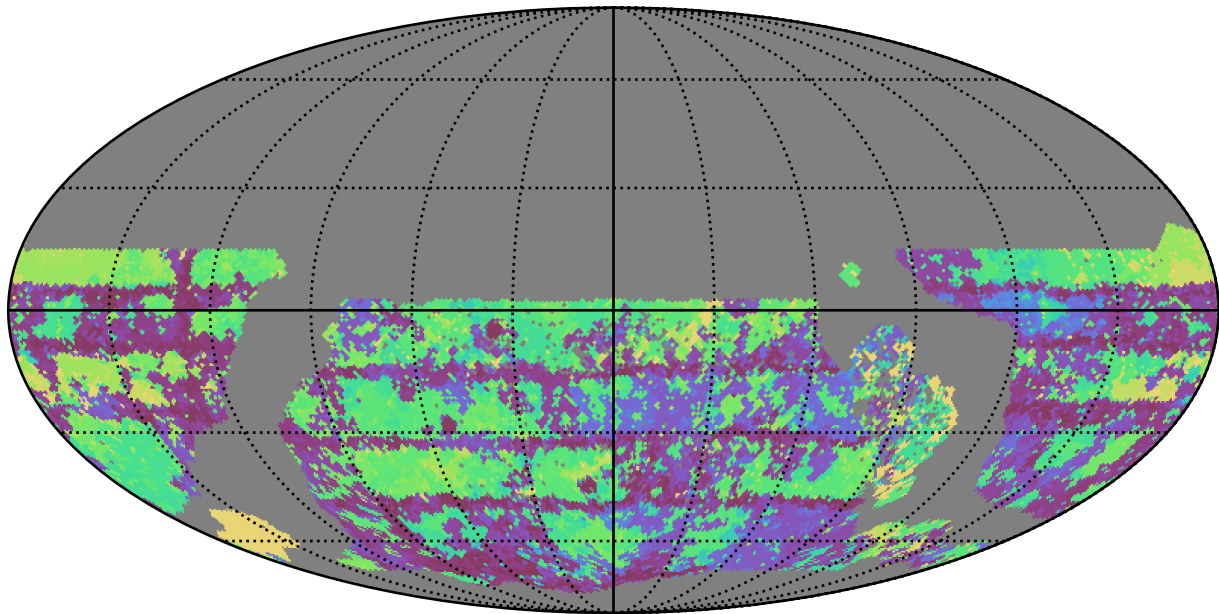
too_100_4v3.4_10yrs WFD u band: Max Inter-Night Gap
