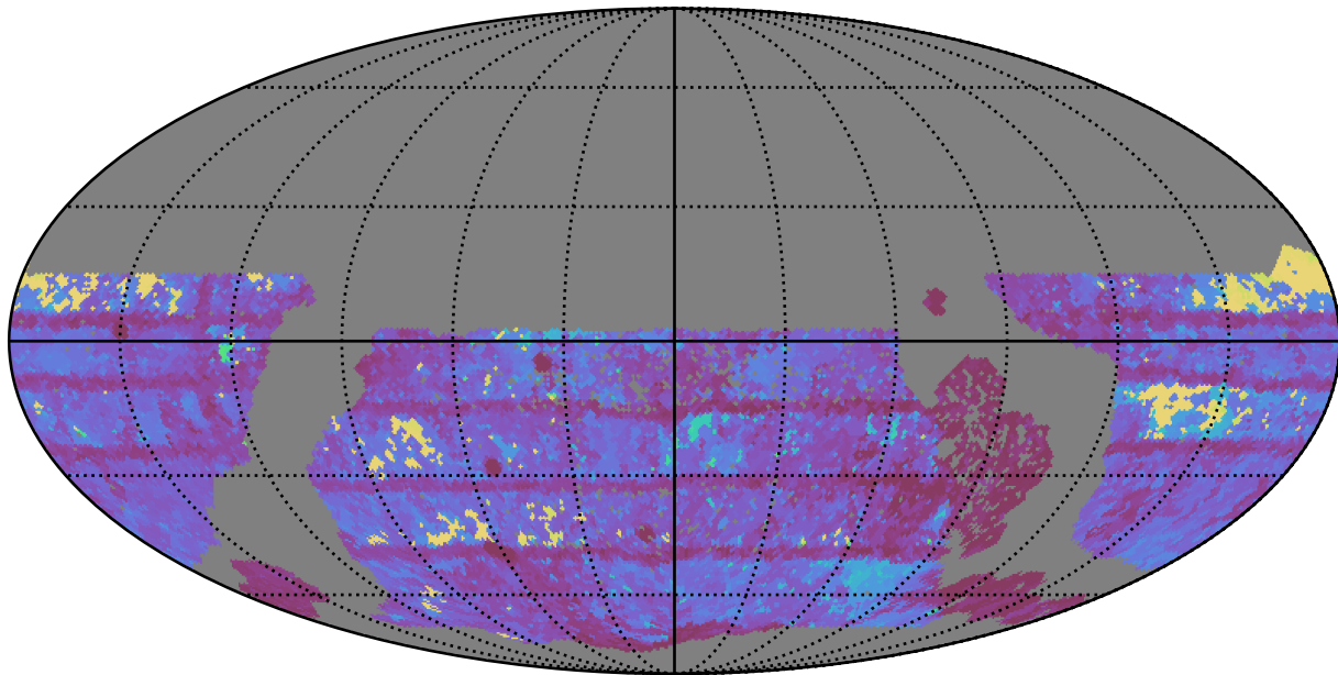
too_100_4v3.4_10yrs WFD r band: Max Inter-Night Gap
