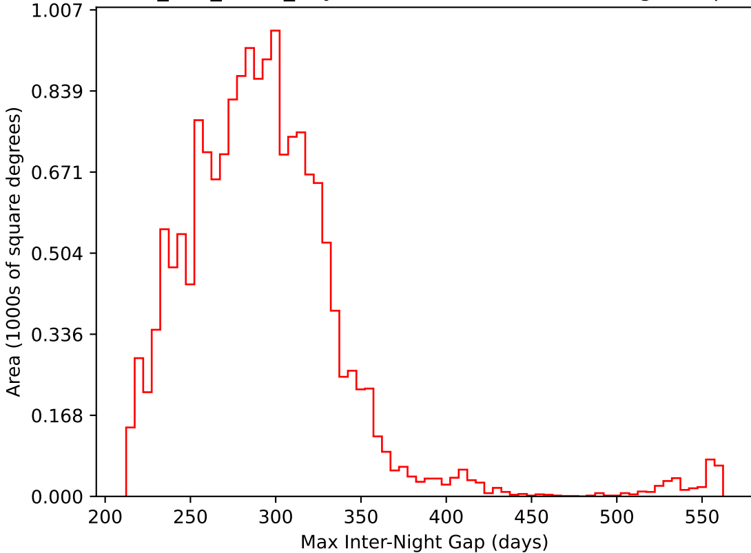
too_100_4v3.4_10yrs WFD i band: Max Inter-Night Gap
