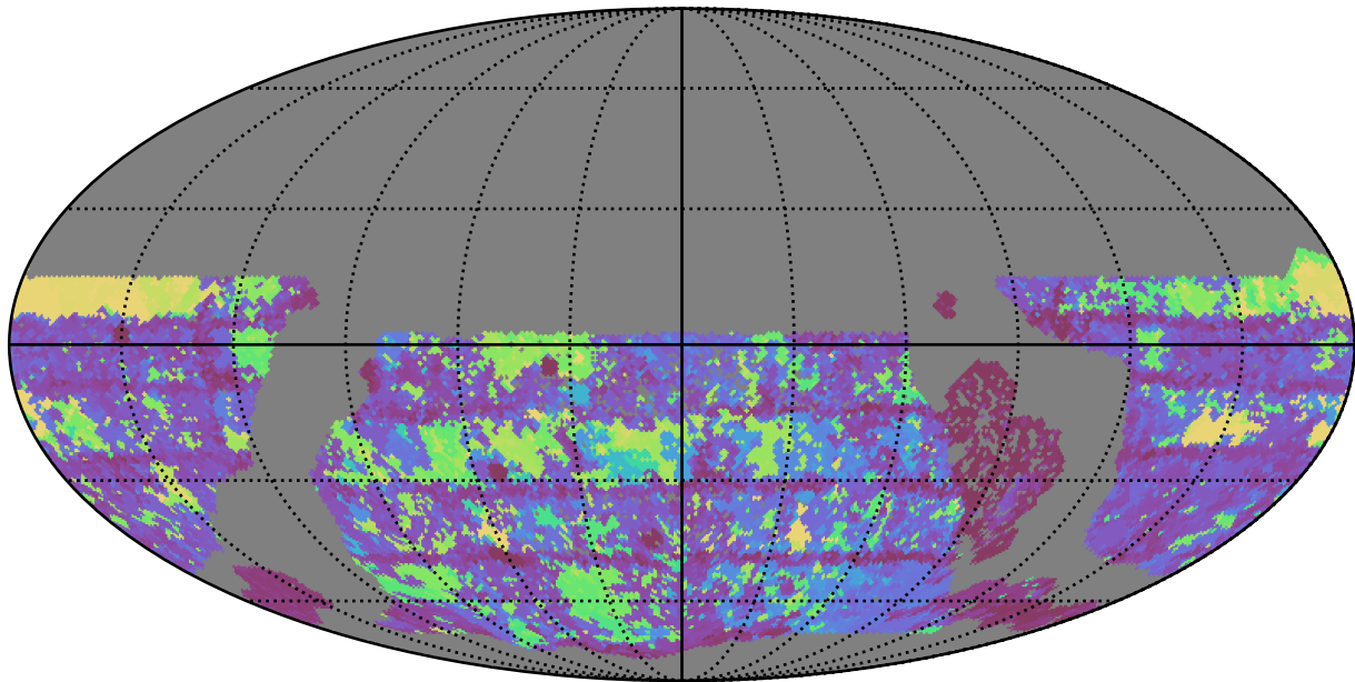
too_100_4v3.4_10yrs WFD g band: Max Inter-Night Gap
