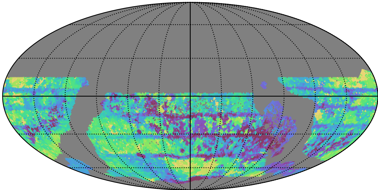
too_100_4v3.4_10yrs WFD all bands: Max Inter-Night Gap
