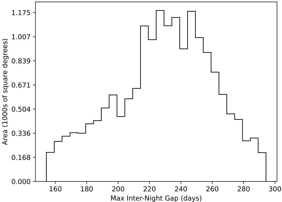
too_100_4v3.4_10yrs WFD all bands: Max Inter-Night Gap
