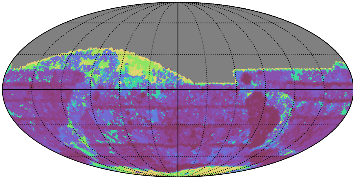
too_100_4v3.4_10yrs All sky z band: Max Inter-Night Gap
