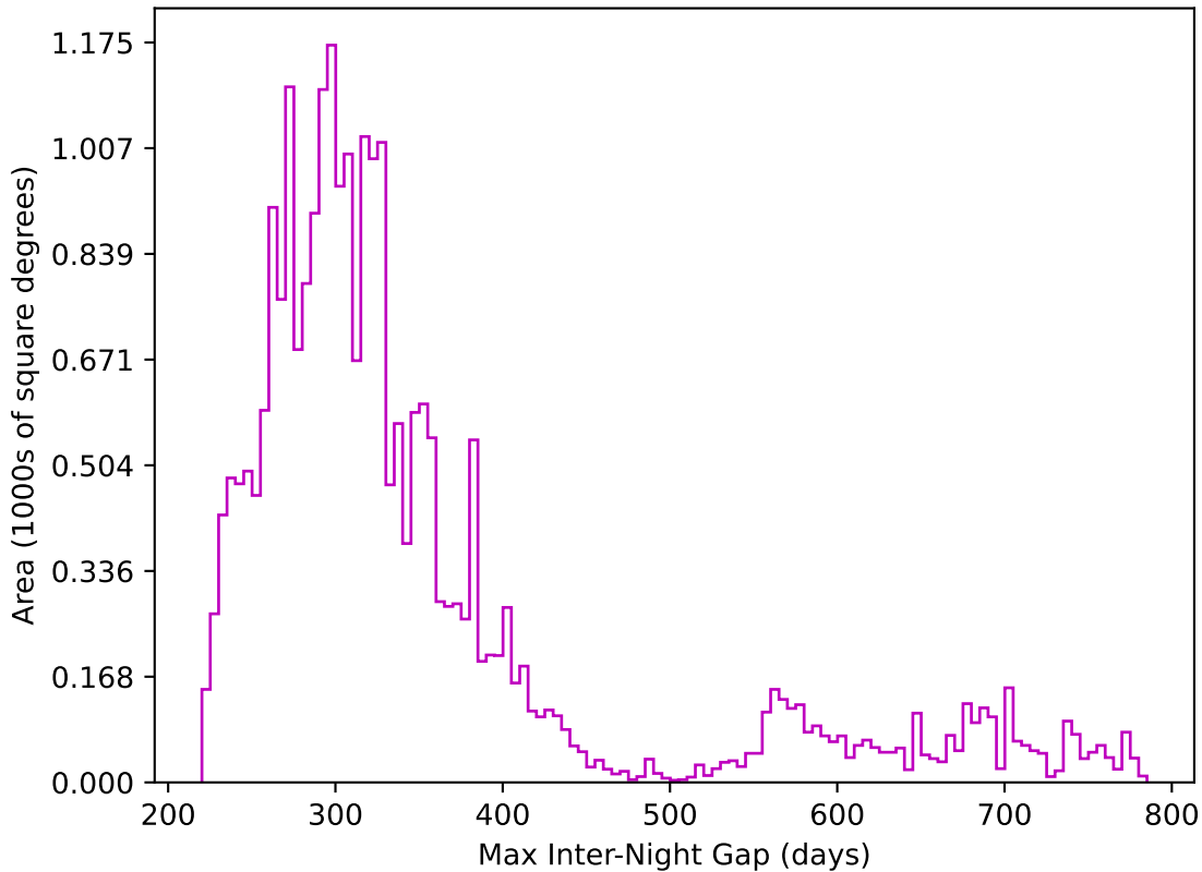
too_100_4v3.4_10yrs All sky z band: Max Inter-Night Gap
