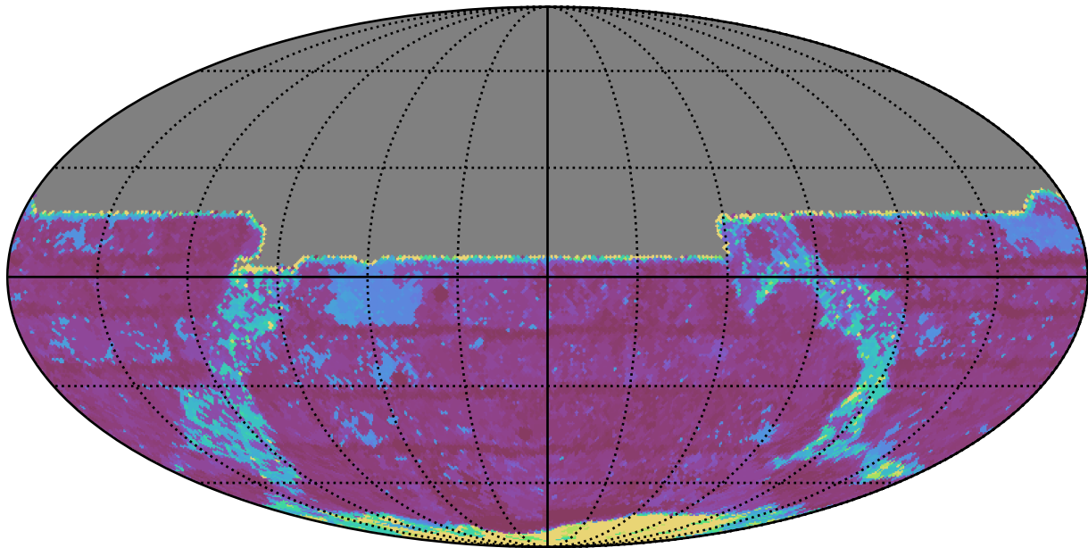
too_100_4v3.4_10yrs All sky y band: Max Inter-Night Gap
