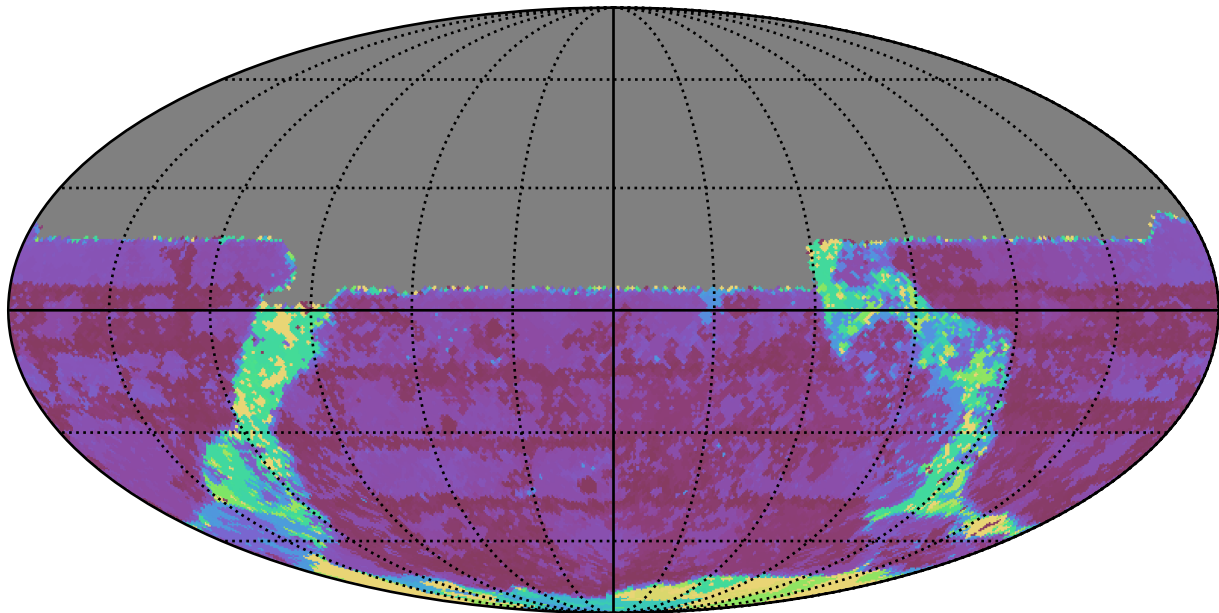
too_100_4v3.4_10yrs All sky u band: Max Inter-Night Gap
