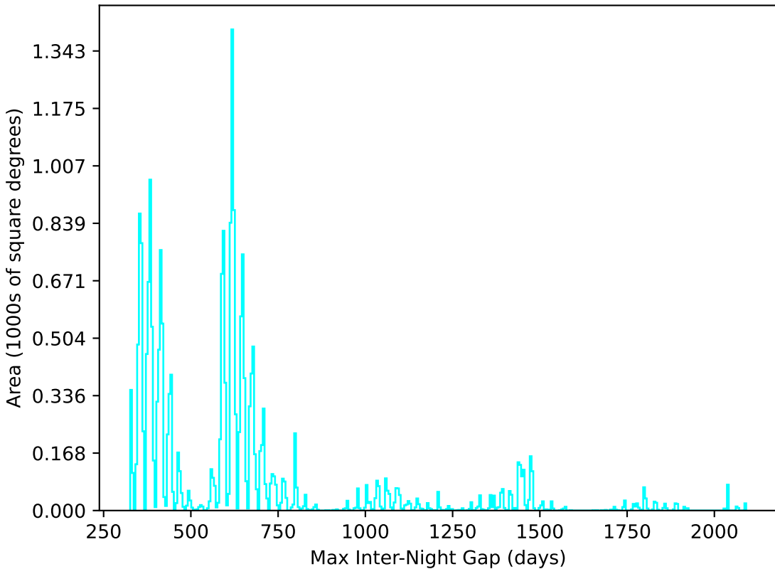
too_100_4v3.4_10yrs All sky u band: Max Inter-Night Gap
