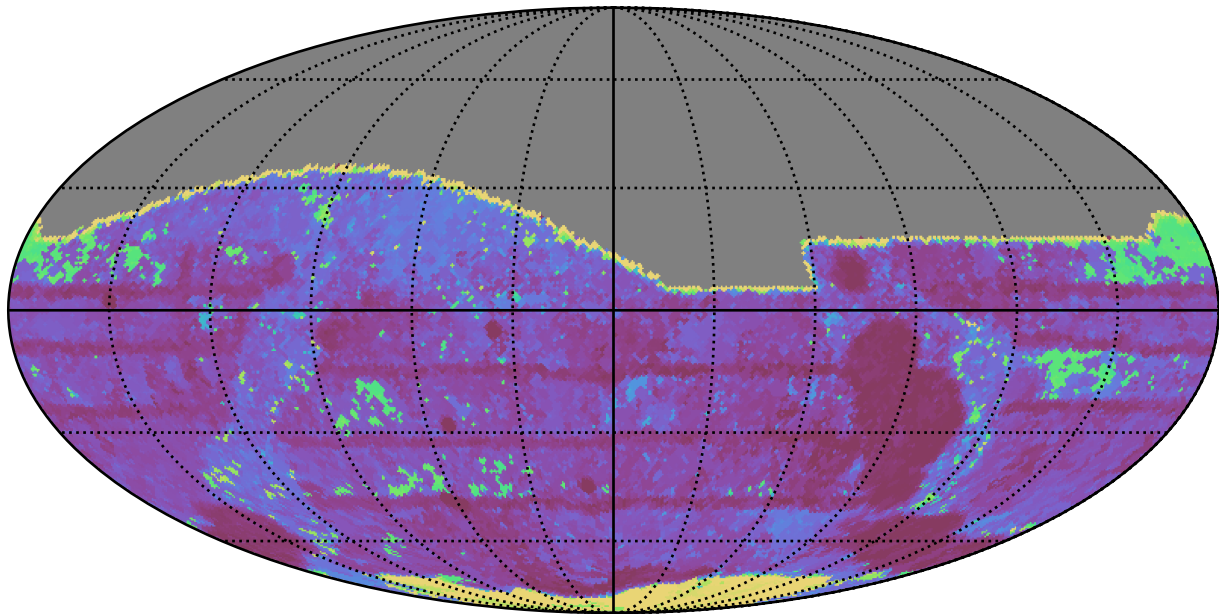
too_100_4v3.4_10yrs All sky r band: Max Inter-Night Gap
