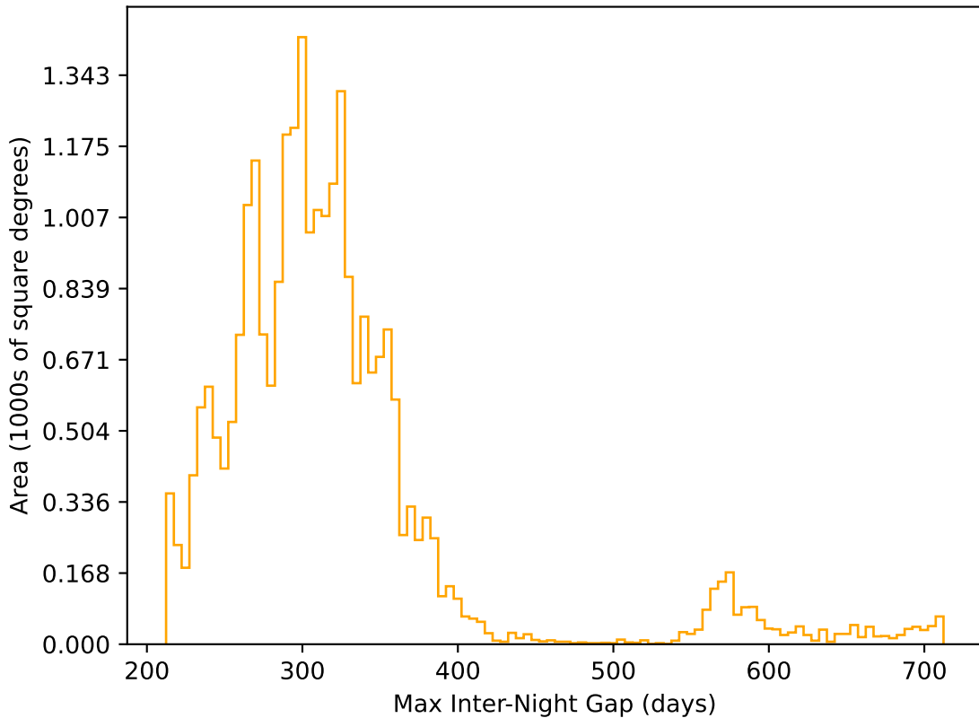
too_100_4v3.4_10yrs All sky r band: Max Inter-Night Gap
