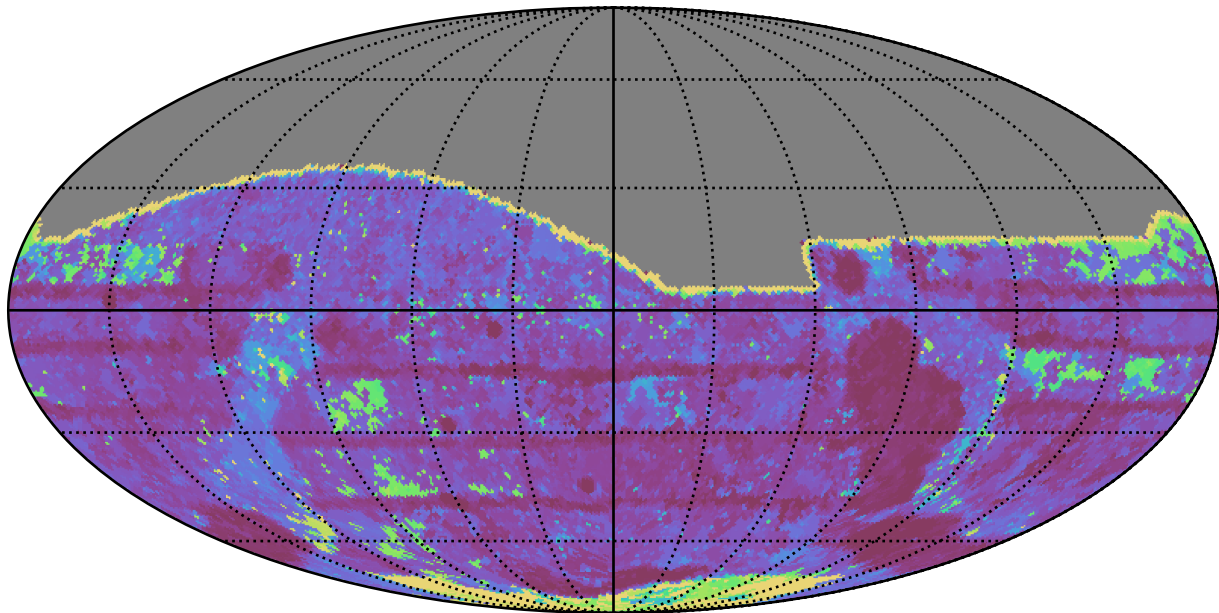
too_100_4v3.4_10yrs All sky i band: Max Inter-Night Gap
