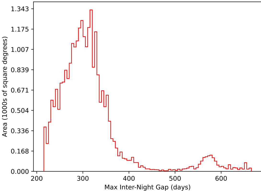
too_100_4v3.4_10yrs All sky i band: Max Inter-Night Gap
