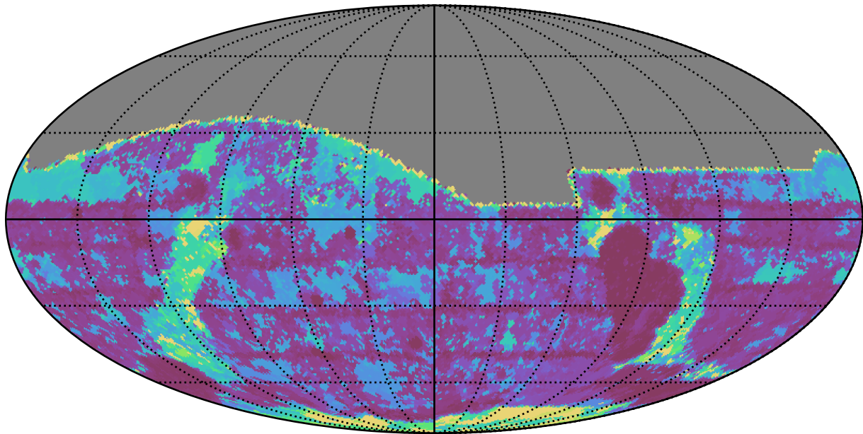
too_100_4v3.4_10yrs All sky g band: Max Inter-Night Gap
