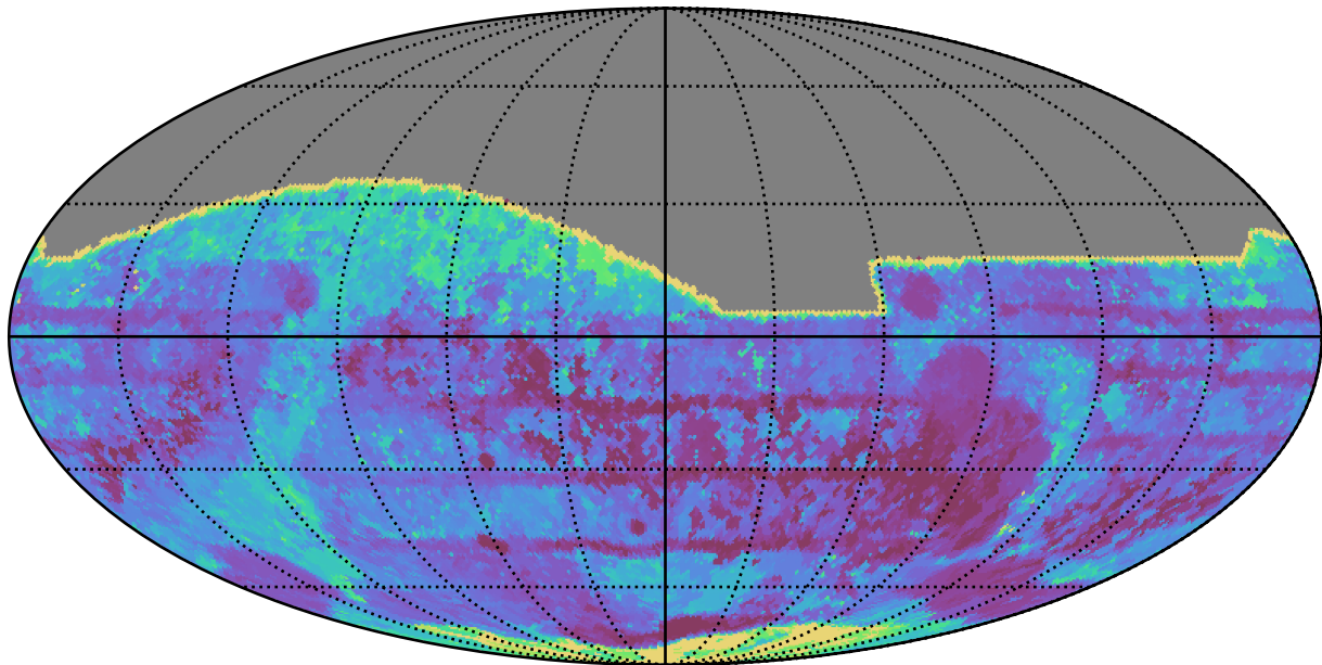
too_100_4v3.4_10yrs All sky all bands: Max Inter-Night Gap
