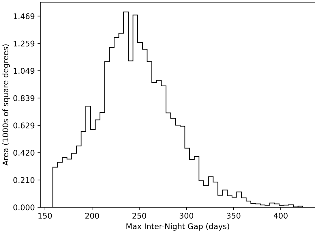
too_100_4v3.4_10yrs All sky all bands: Max Inter-Night Gap
