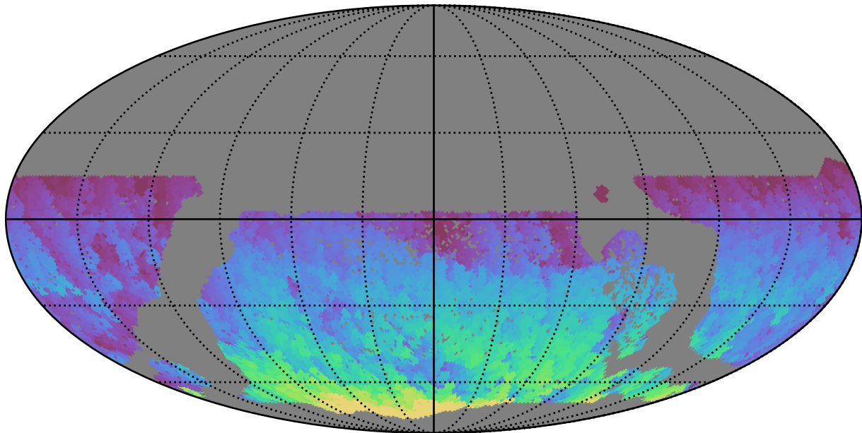
too_100_4v3.4_10yrs WFD z band: Max HA
