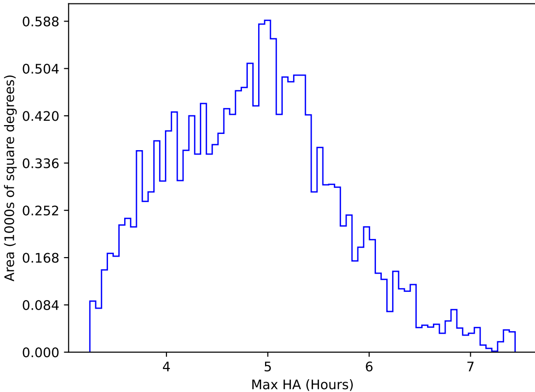
too_100_4v3.4_10yrs WFD z band: Max HA
