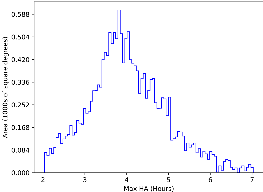
too_100_4v3.4_10yrs WFD u band: Max HA
