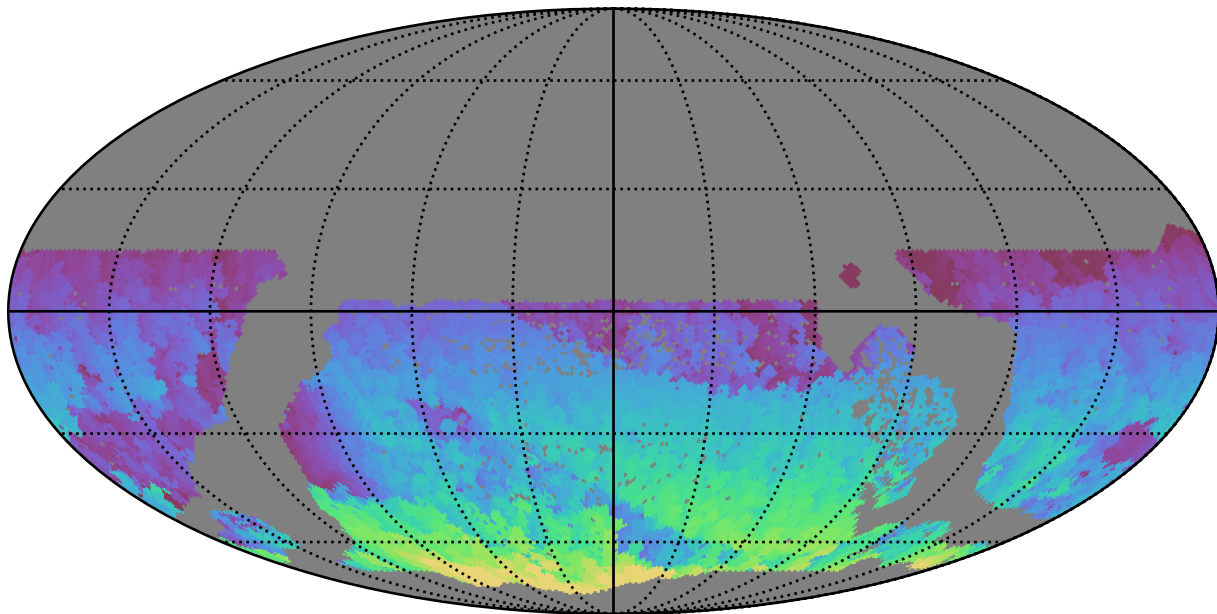
too_100_4v3.4_10yrs WFD i band: Max HA
