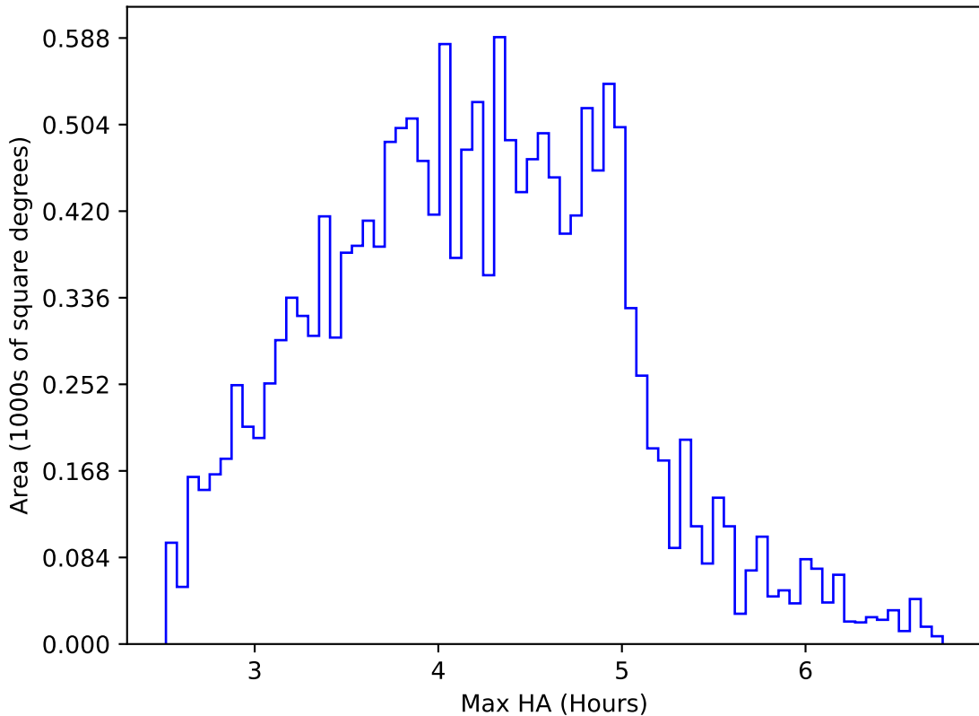
too_100_4v3.4_10yrs WFD g band: Max HA
