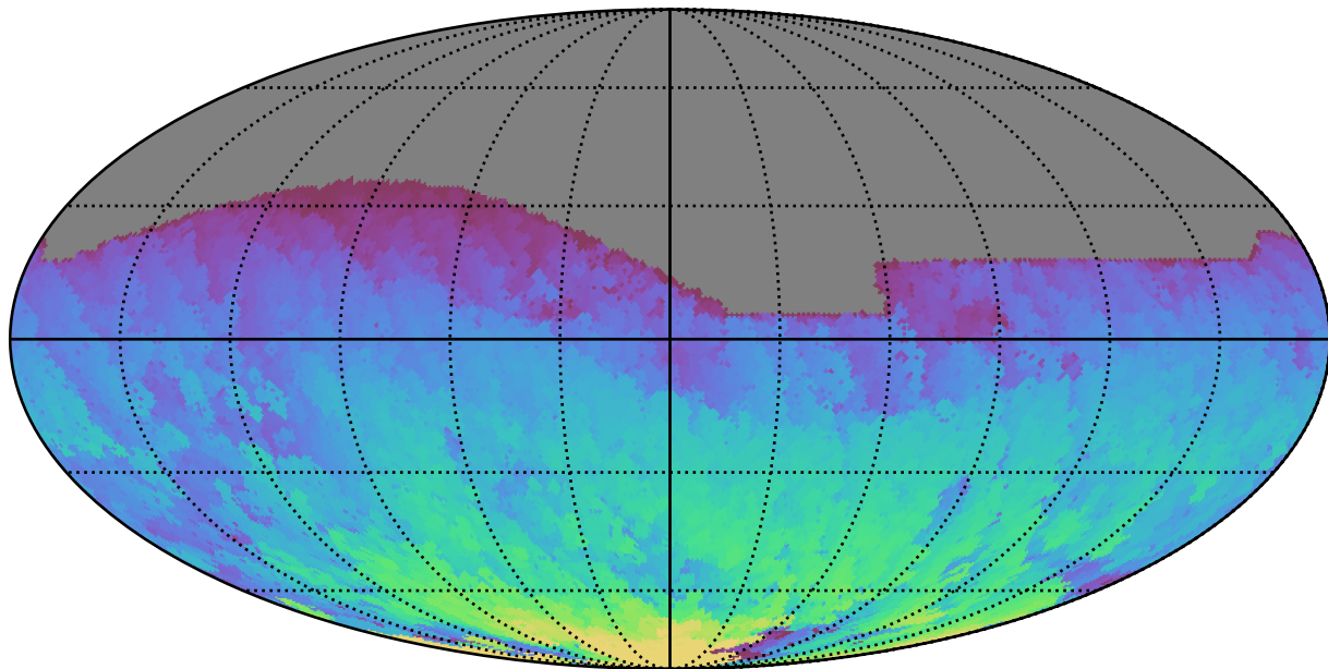
too_100_4v3.4_10yrs All sky z band: Max HA
